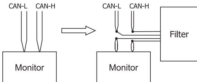
Fig. 3. Full duplex CAN bus breakage diagram
