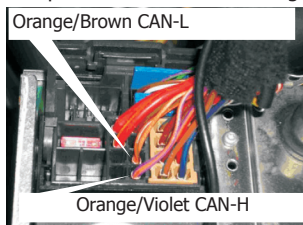
Fig. 2. CAN bus contacts location in monitor's port in VW Touareg, VW Multivan T5, VW Passat B6 vehicles.
